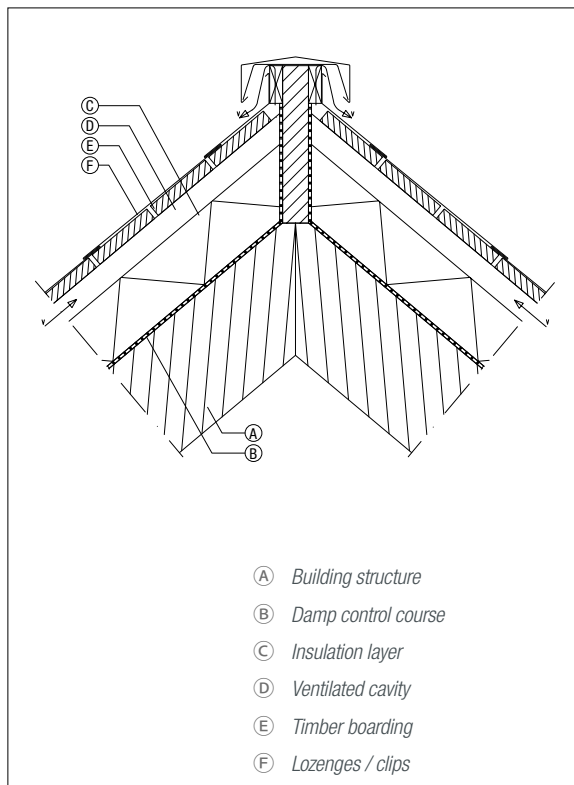
Figure 6.3.6 Ridge detail
