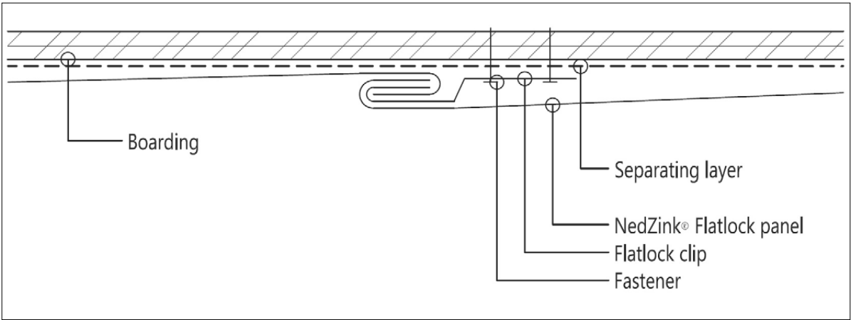
Figure 7.3.2 Flatlock Horizontal Section
