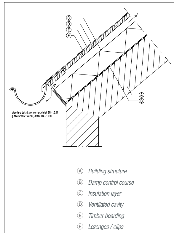
Figure 6.3.7 Gutter detail
