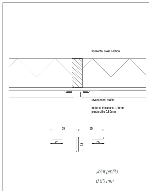
Figure 7.2.3 Joint profiles.
