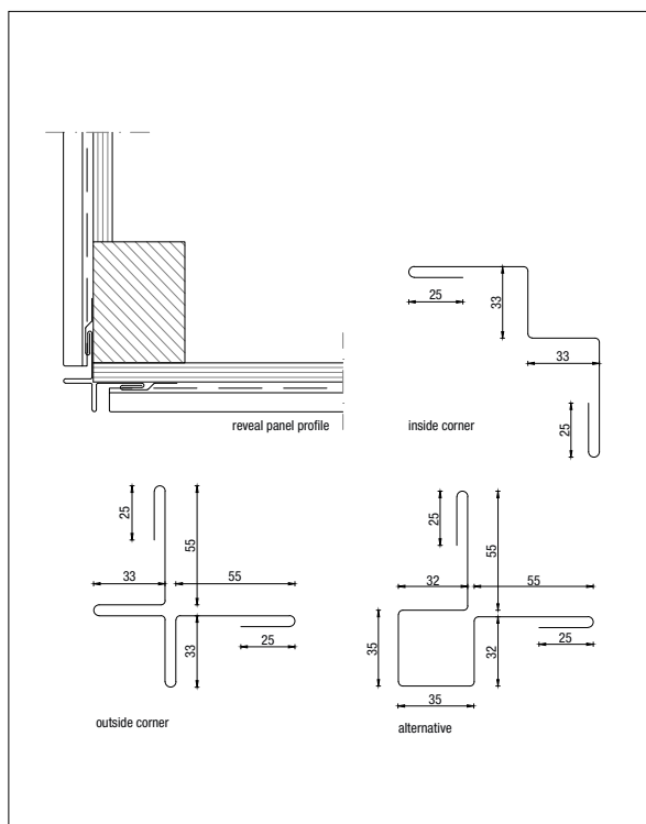
Figure 7.2.2 Connection profiles.
