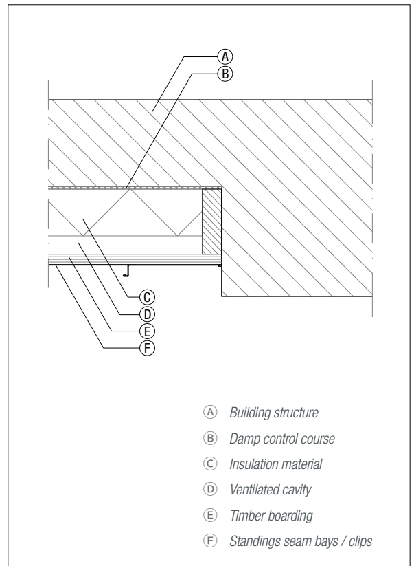
Figure 7.1.11 Wall abutment
