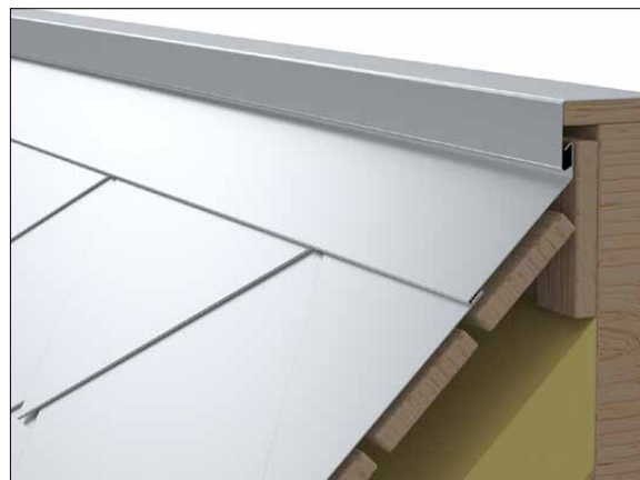
Figure 6.3.13 Details lozenge system on a ventilated substructure.
